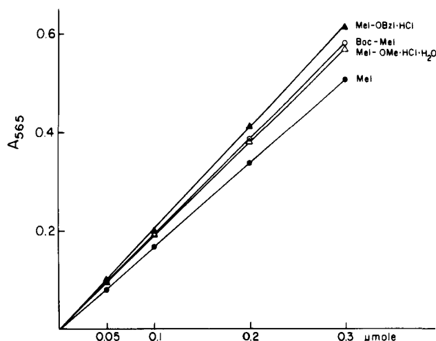
Figure 1. Determination of Mel, Mel-OMe·HCl·H 2 O (1), Mel-OBz·HCl (2), and Boc-Mel (3) with 4-( p -nitrobenzyl)pyridine.
